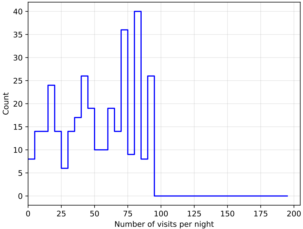
scp_reweight_v3.3_10yrs all bands: DD:EDFS NVisitsPerNight
