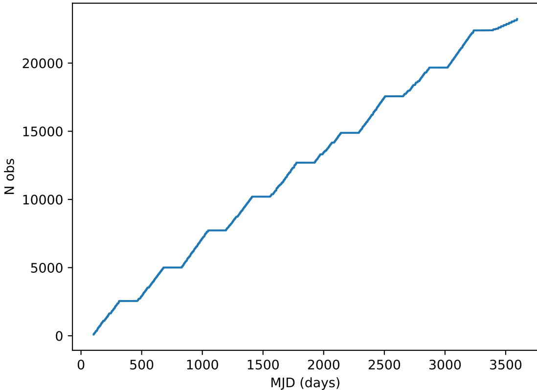
scp_reweight_v3.3_10yrs all bands: DD:EDFS Cumulative NVisits
