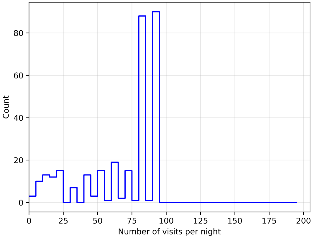
scp_reweight_v3.3_10yrs all bands: DD:ECDFS NVisitsPerNight
