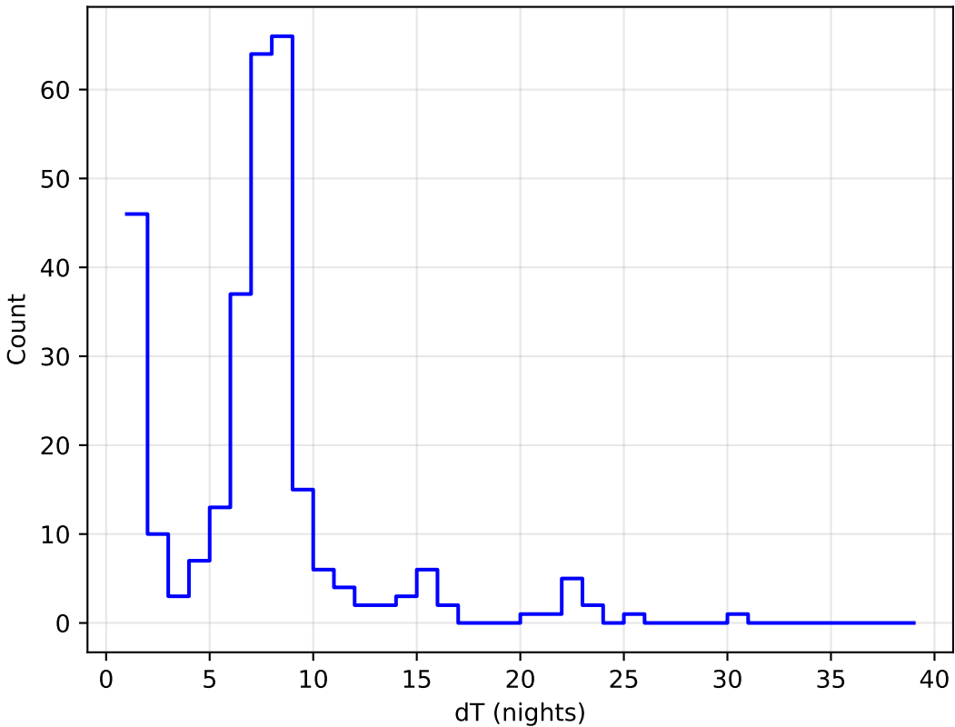
scp_reweight_v3.3_10yrs all bands: DD:ECDFS Delta Nights Histogram
