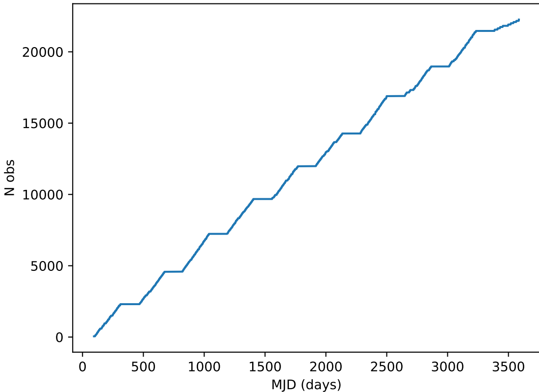
scp_reweight_v3.3_10yrs all bands: DD:ECDFS Cumulative NVisits
