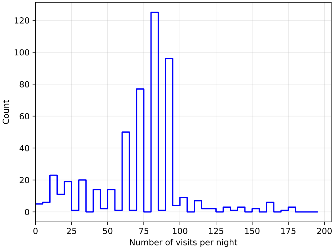
scp_reweight_v3.3_10yrs all bands: DD:COSMOS NVisitsPerNight
