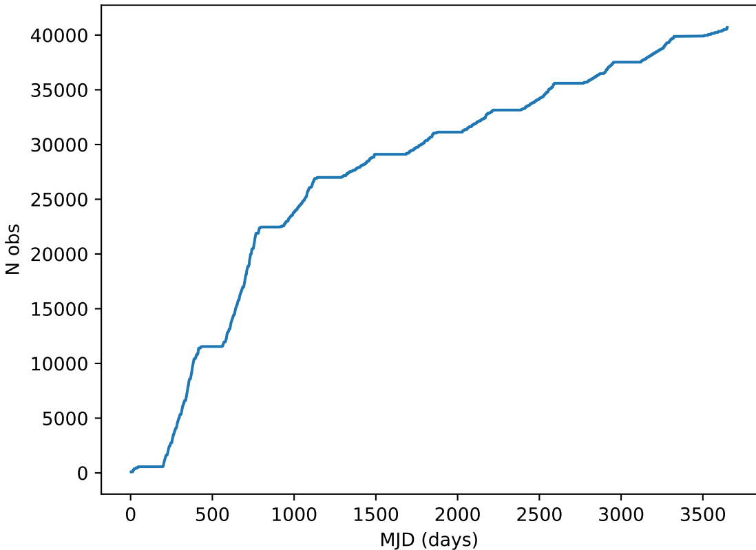
scp_reweight_v3.3_10yrs all bands: DD:COSMOS Cumulative NVisits
