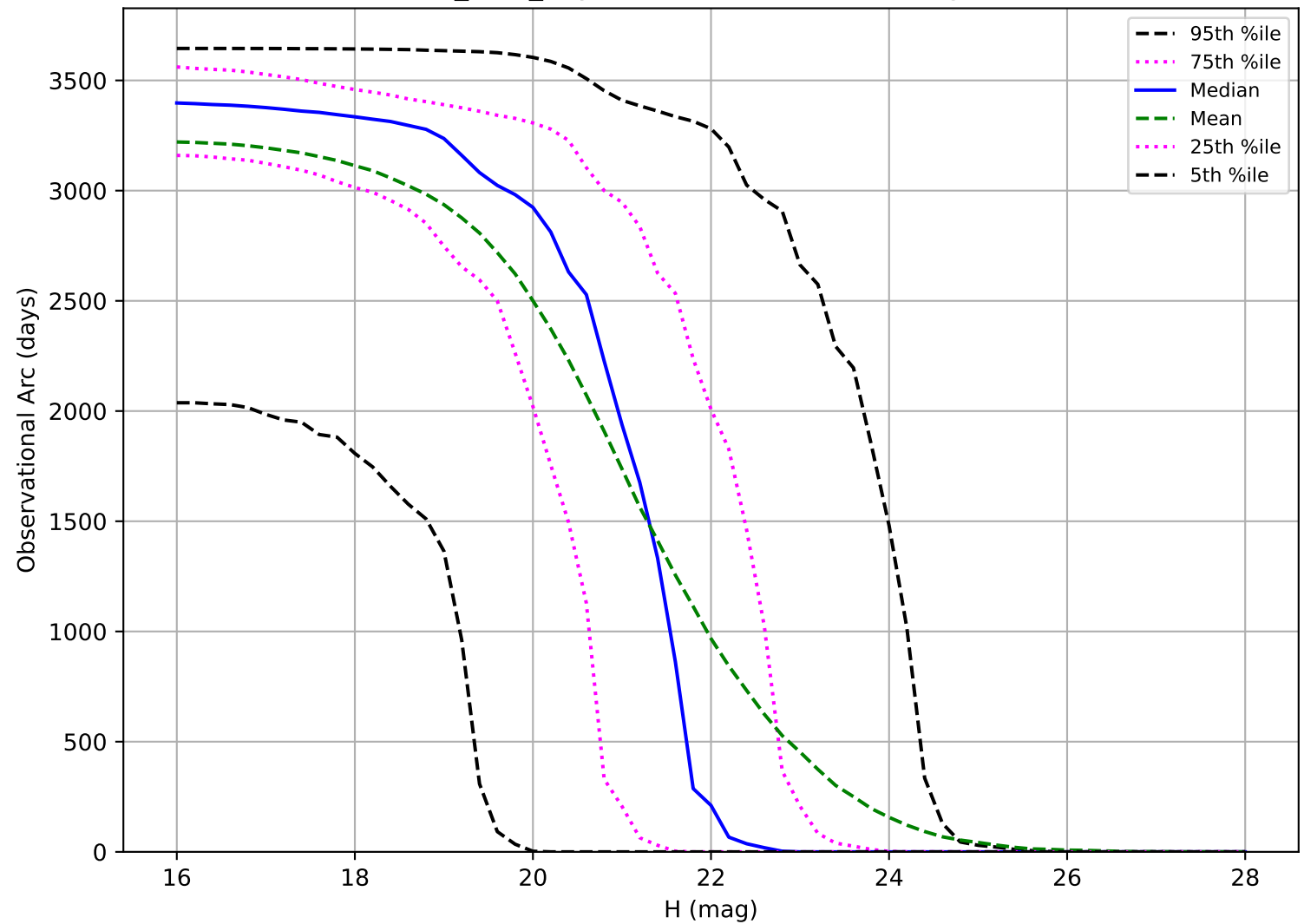
roman_v3.3_10yrs: Observational Arc Length PHA
