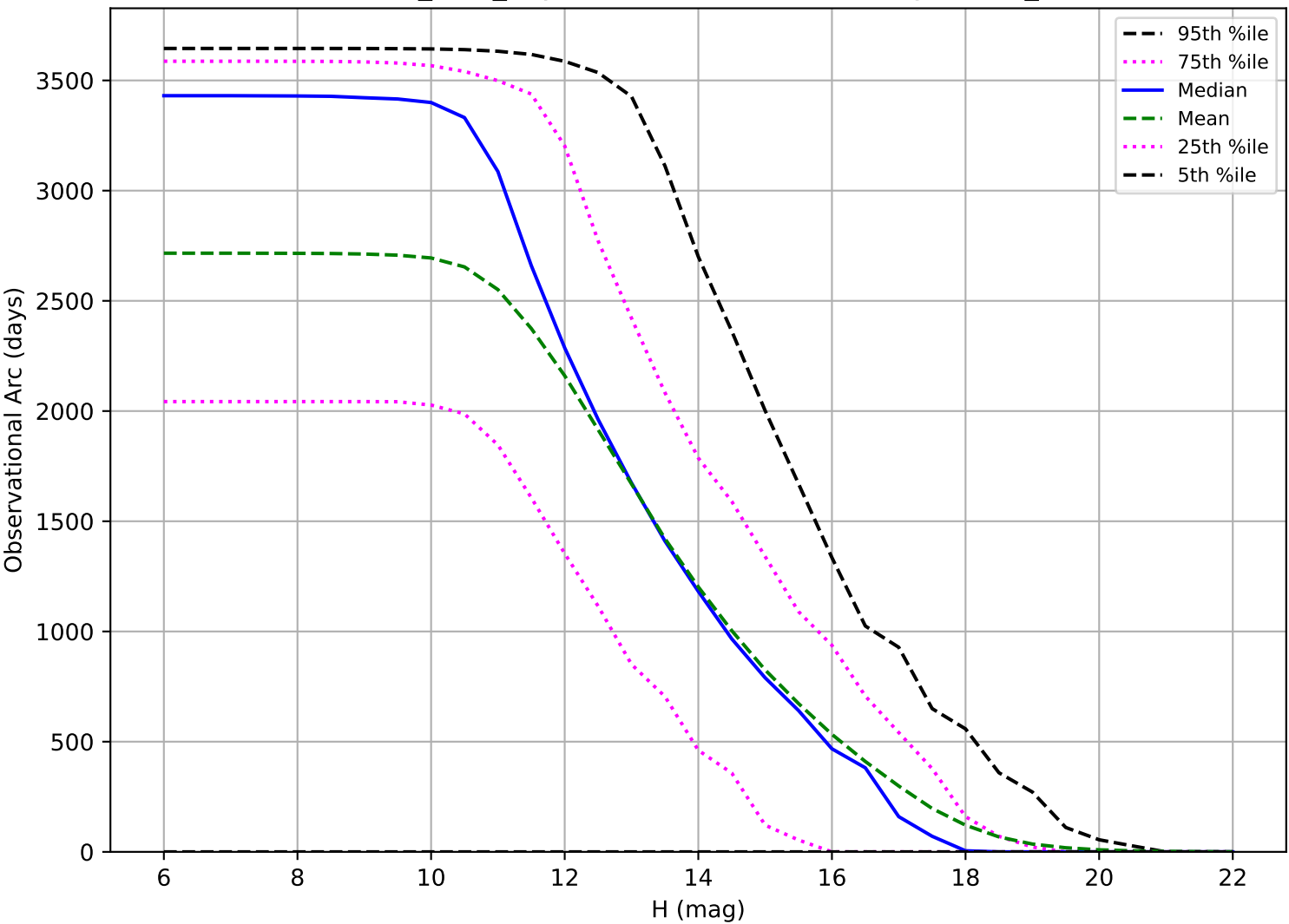
roman_v3.3_10yrs: Observational Arc Length OCC_r5
