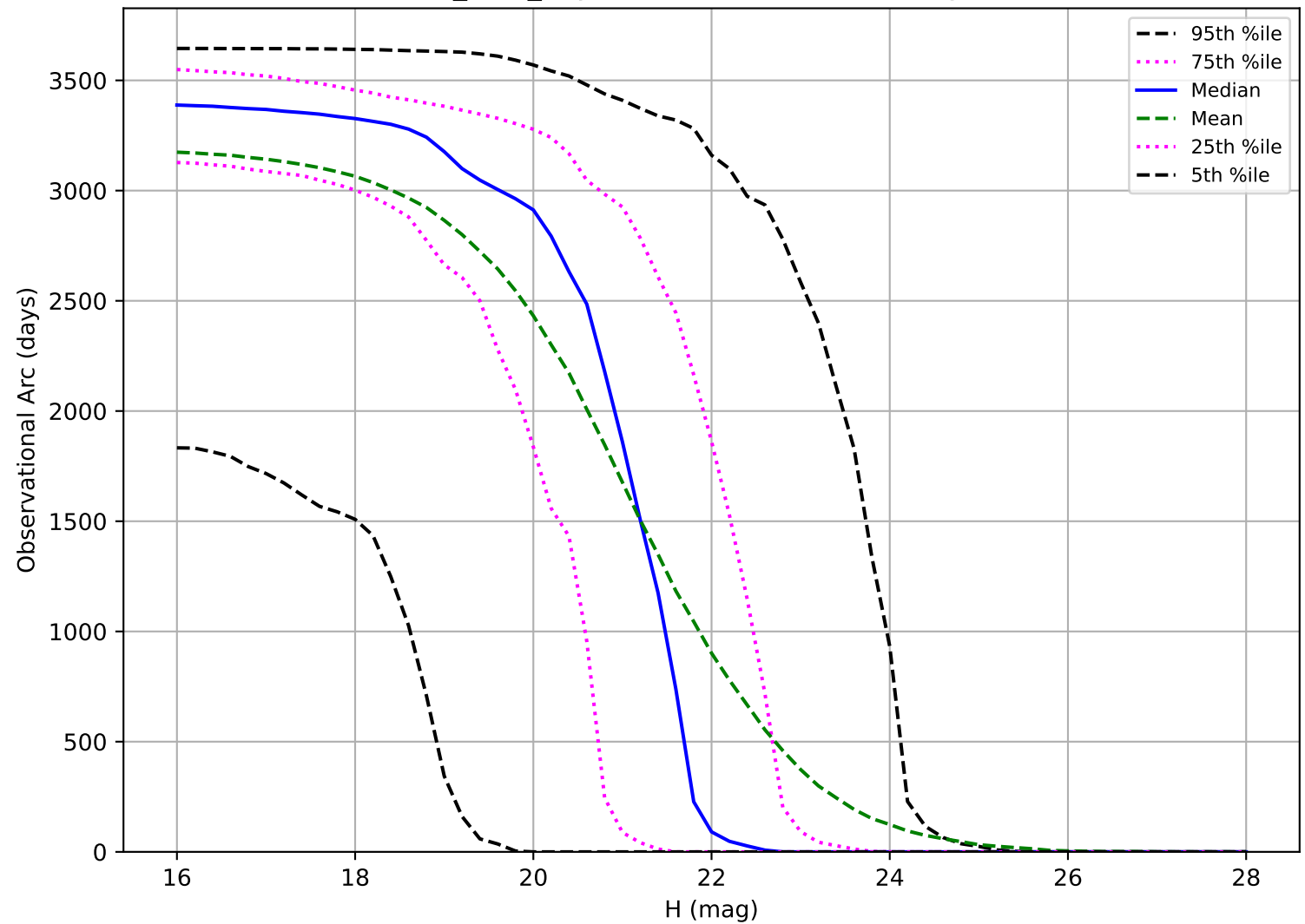
roman_v3.3_10yrs: Observational Arc Length NEO
