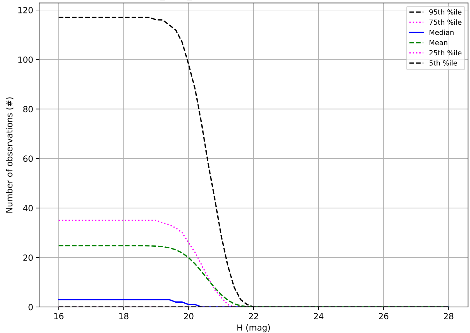
roman_v3.3_10yrs: Number of observations Vatira
