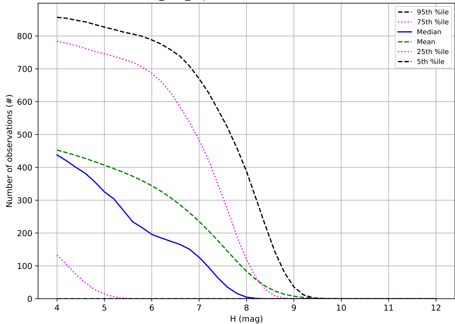
roman_v3.3_10yrs: Number of observations TNO
