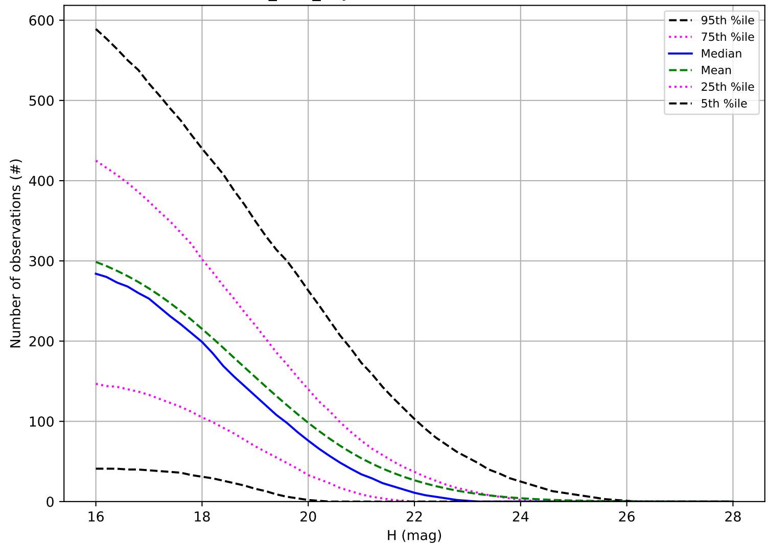
roman_v3.3_10yrs: Number of observations PHA
