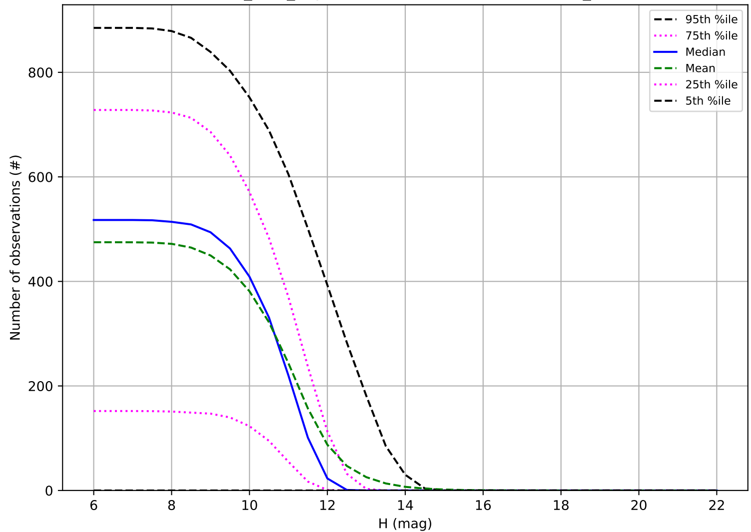
roman_v3.3_10yrs: Number of observations OCC_r20
