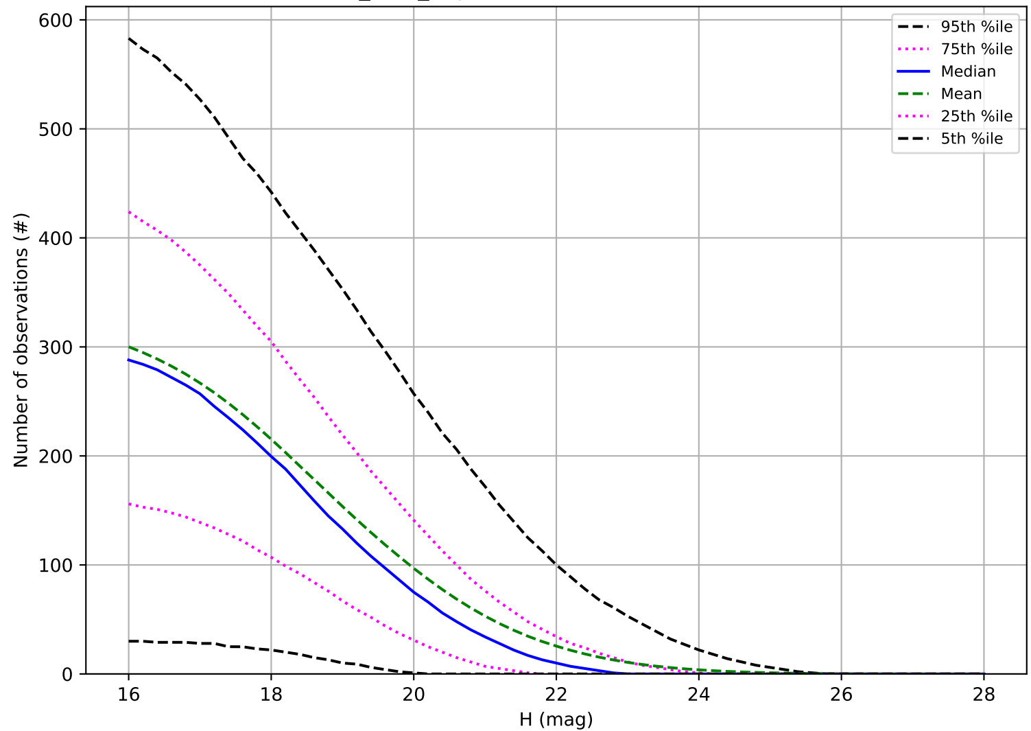
roman_v3.3_10yrs: Number of observations NEO
