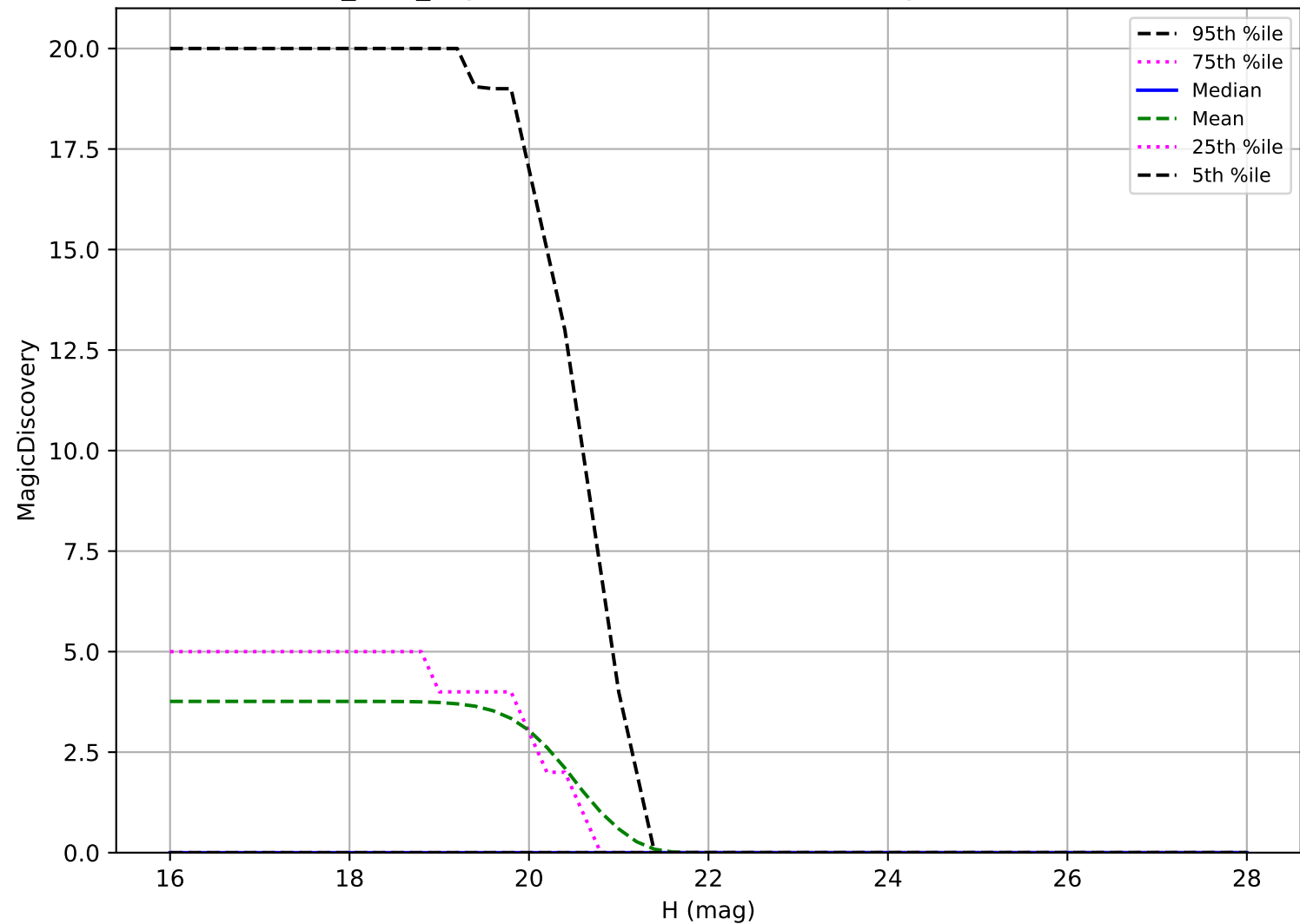
roman_v3.3_10yrs: Vatira 6 detections in 60 nights detection loss
