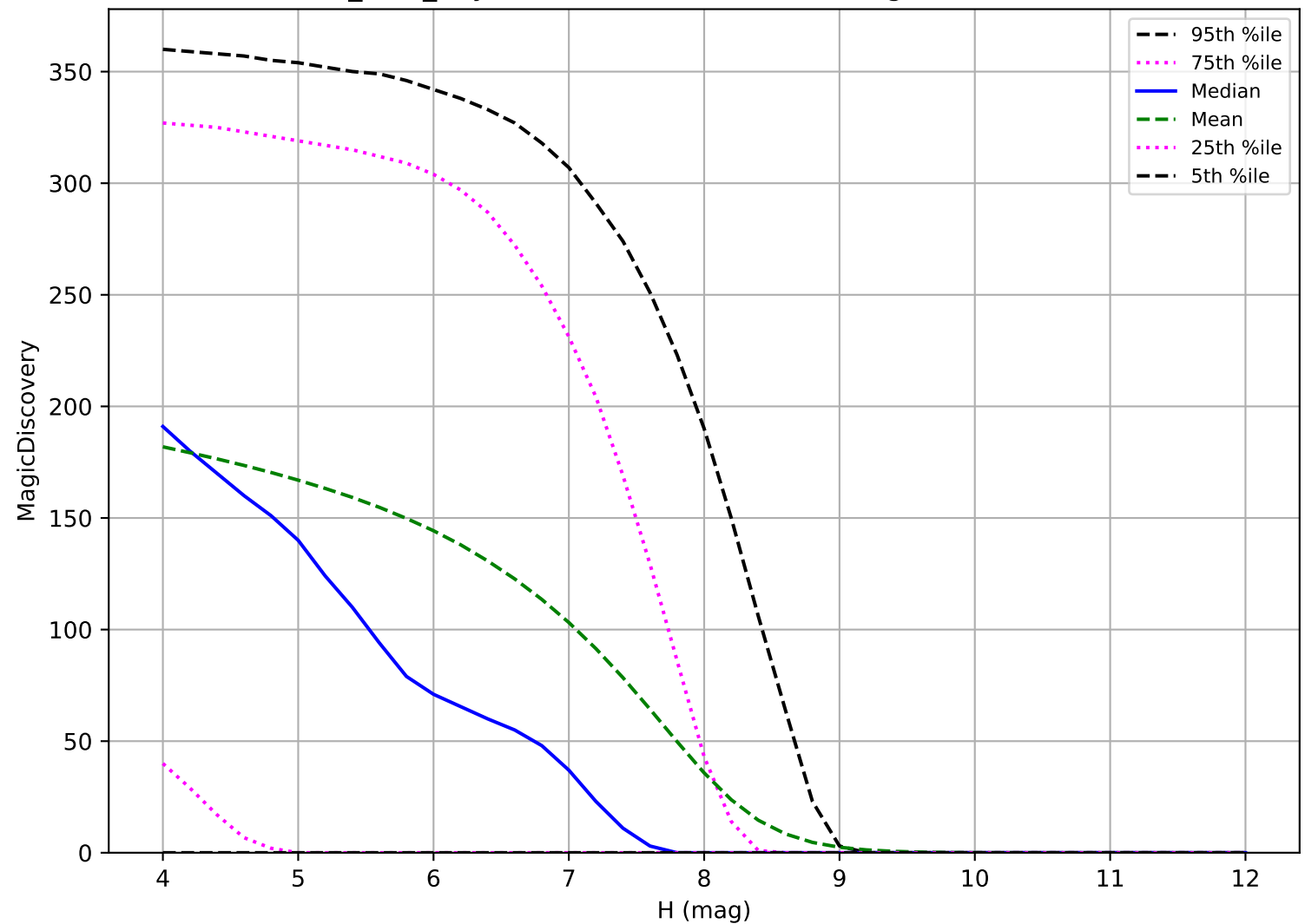
roman_v3.3_10yrs: TNO 6 detections in 60 nights detection loss
