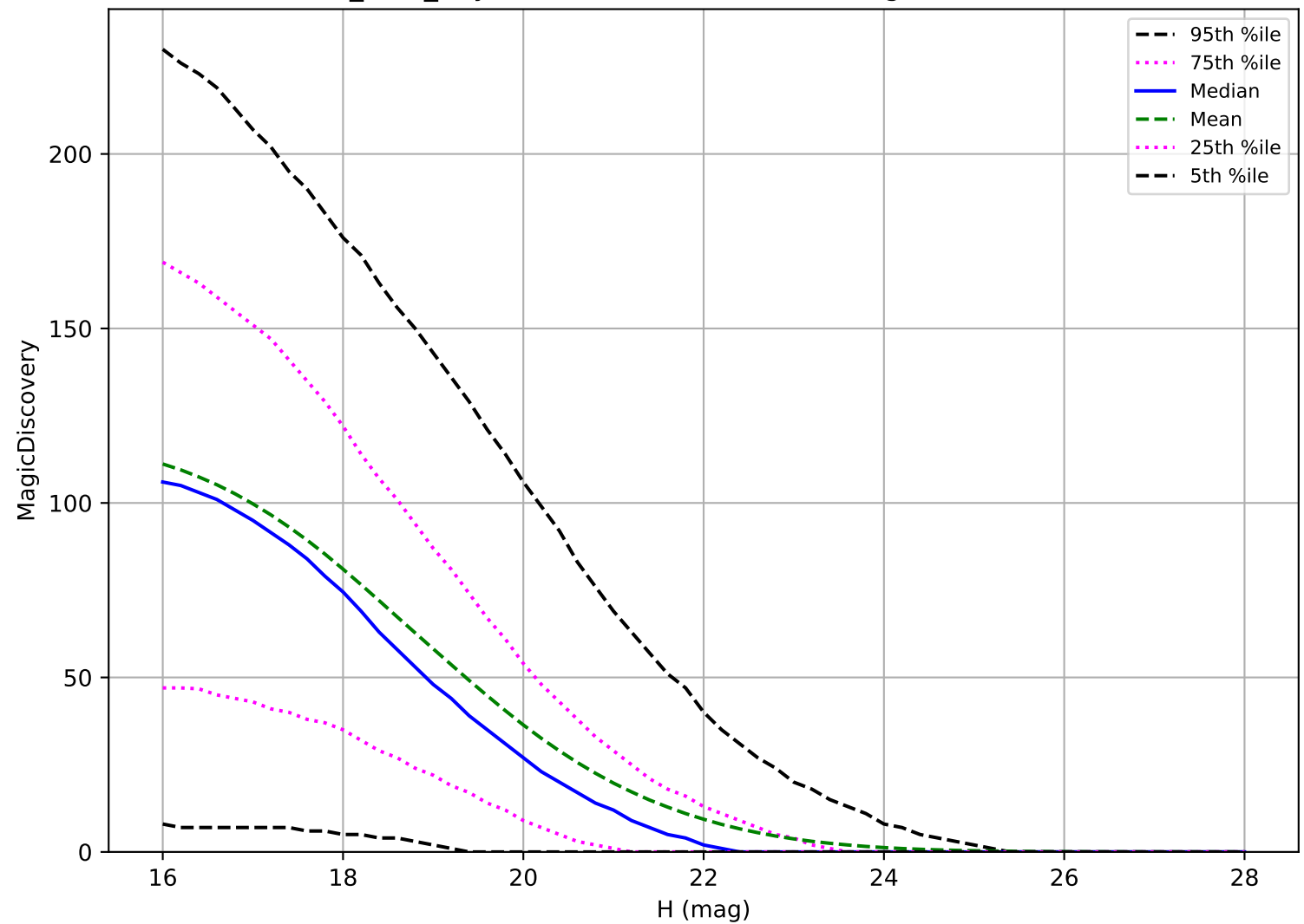
roman_v3.3_10yrs: PHA 6 detections in 60 nights detection loss
