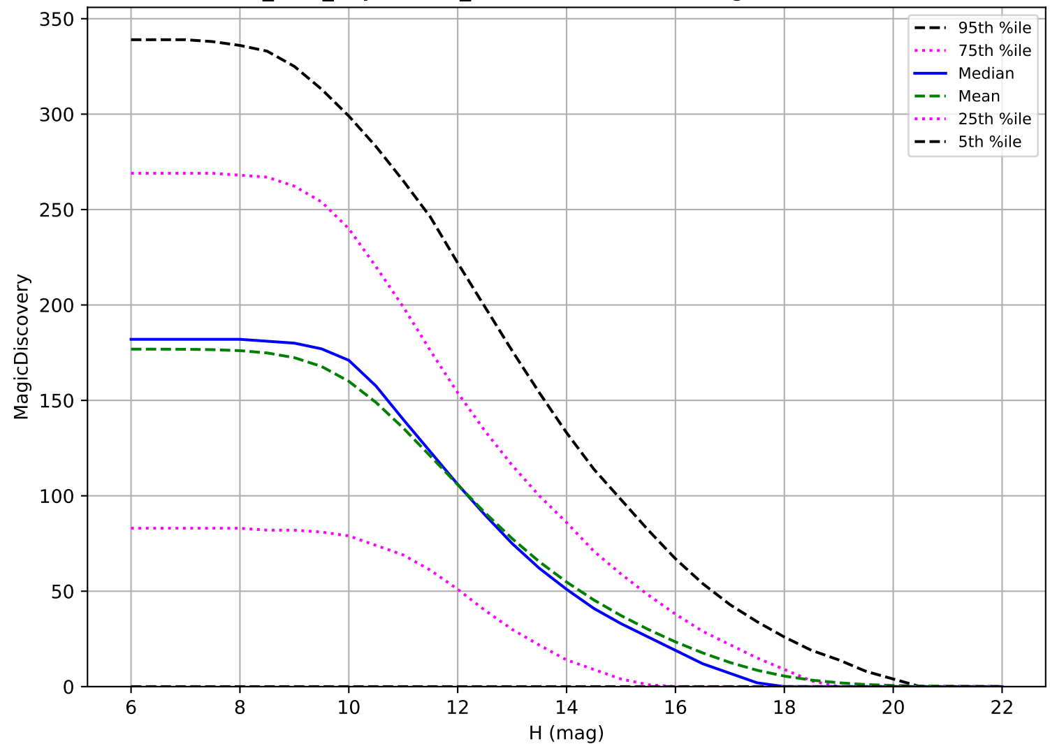
roman_v3.3_10yrs: OCC_r5 6 detections in 60 nights detection loss
