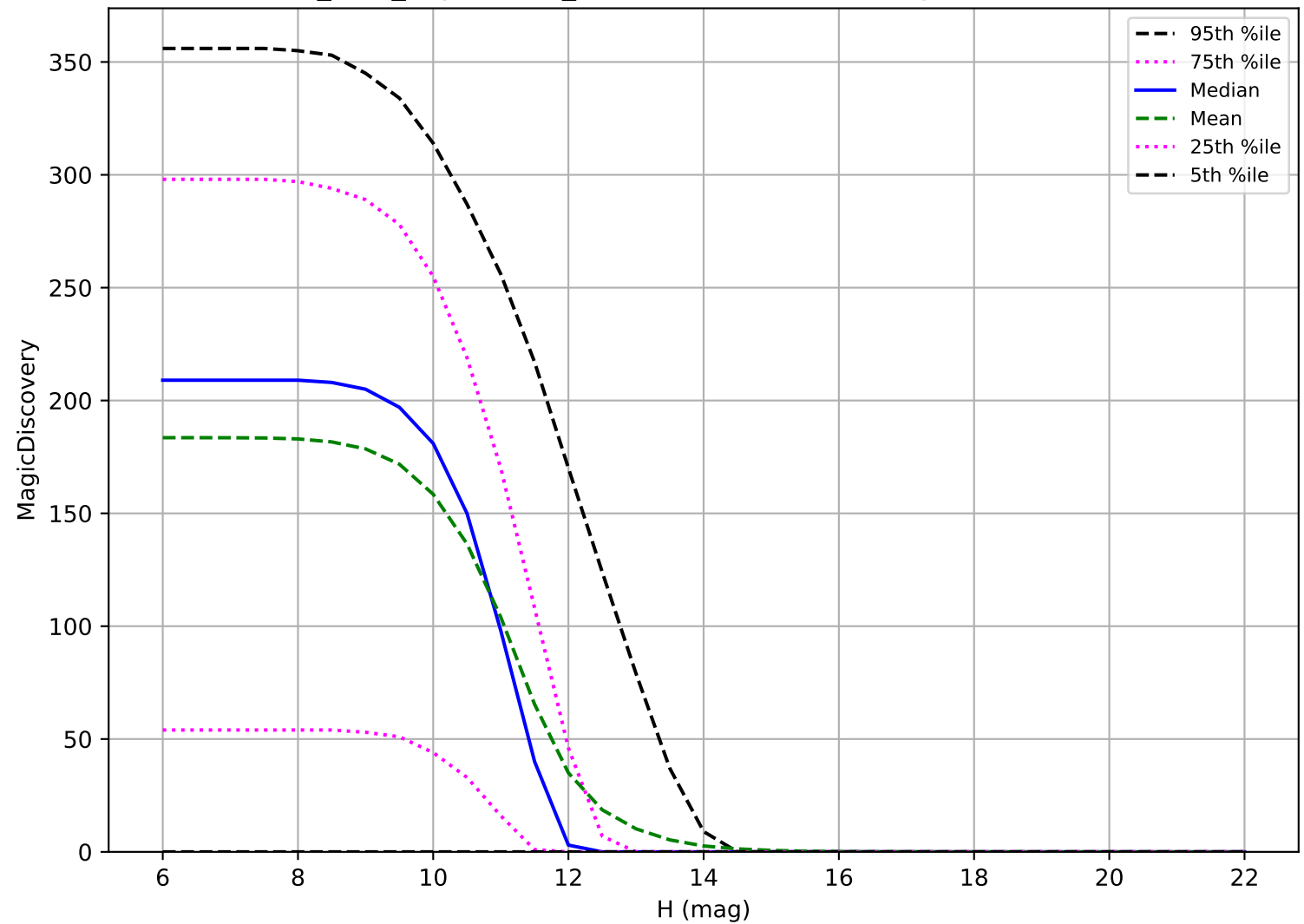
roman_v3.3_10yrs: OCC_r20 6 detections in 60 nights detection loss
