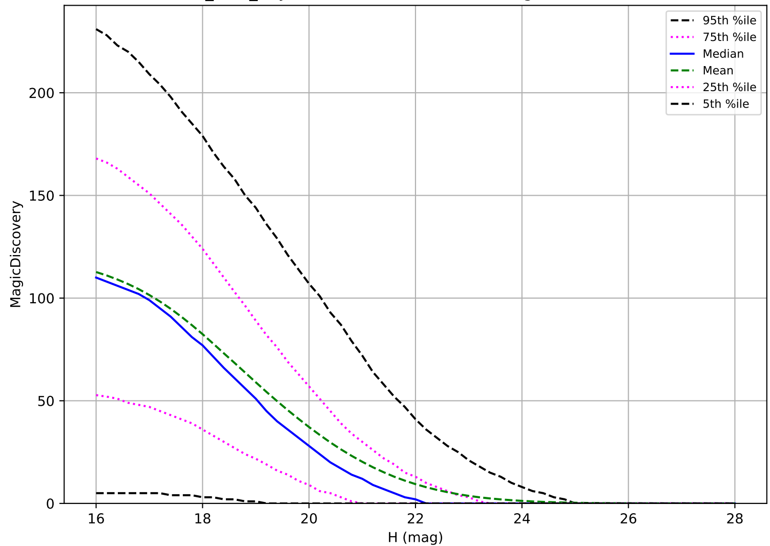
roman_v3.3_10yrs: NEO 6 detections in 60 nights detection loss
