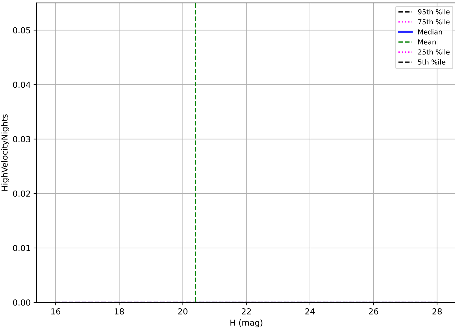
roman_v3.3_10yrs: Vatira High velocity pair detection loss
