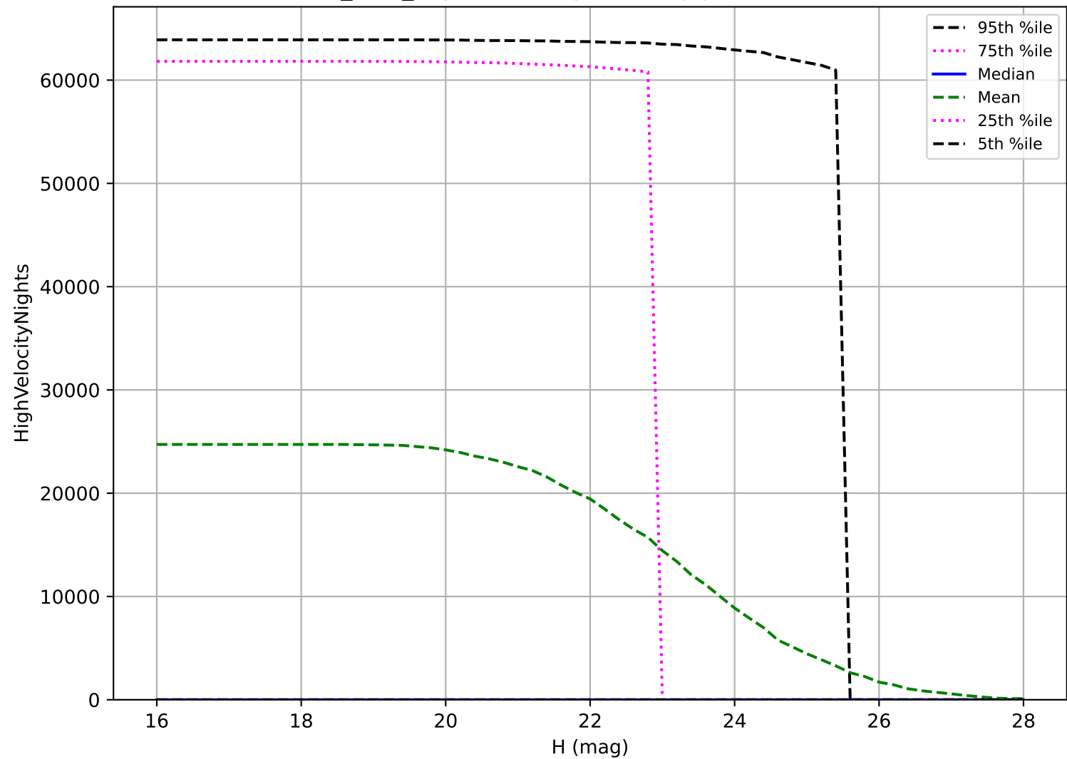
roman_v3.3_10yrs: PHA High velocity pair detection loss
