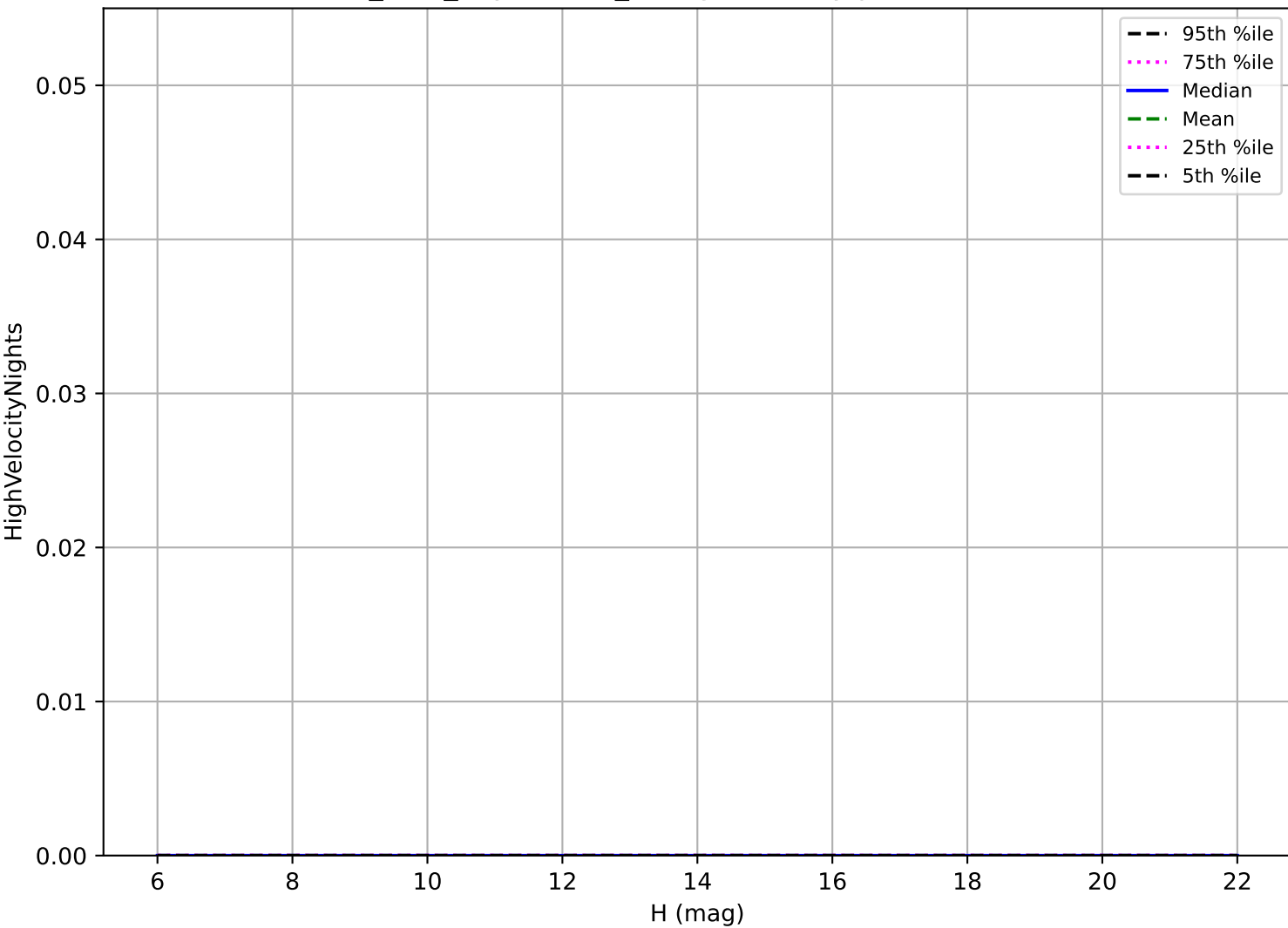
roman_v3.3_10yrs: OCC_r5 High velocity pair detection loss
