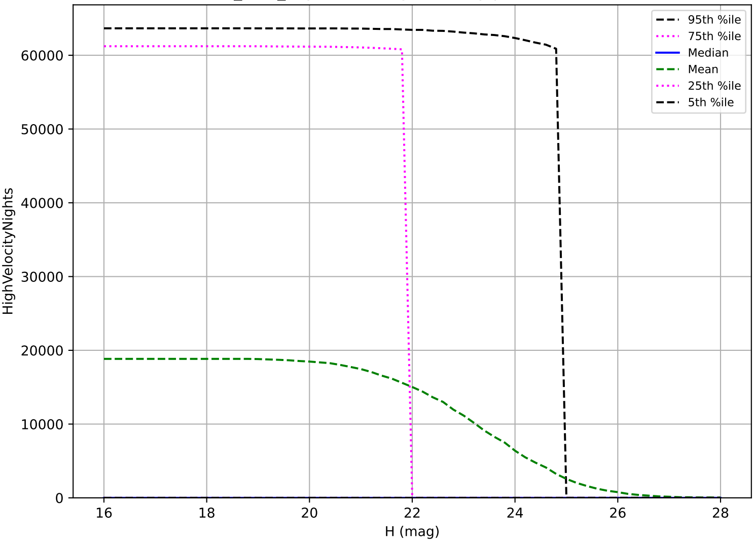
roman_v3.3_10yrs: NEO High velocity pair detection loss
