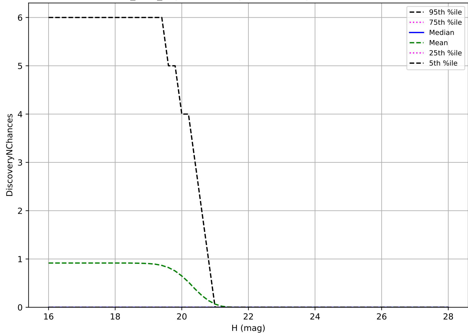
roman_v3.3_10yrs: Vatira 3 pairs in 15 nights detection loss
