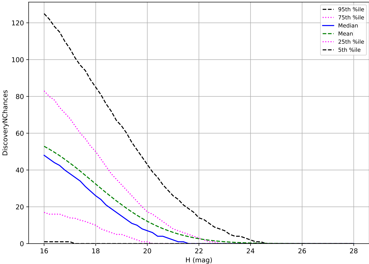
roman_v3.3_10yrs: PHA 3 pairs in 15 nights detection loss
