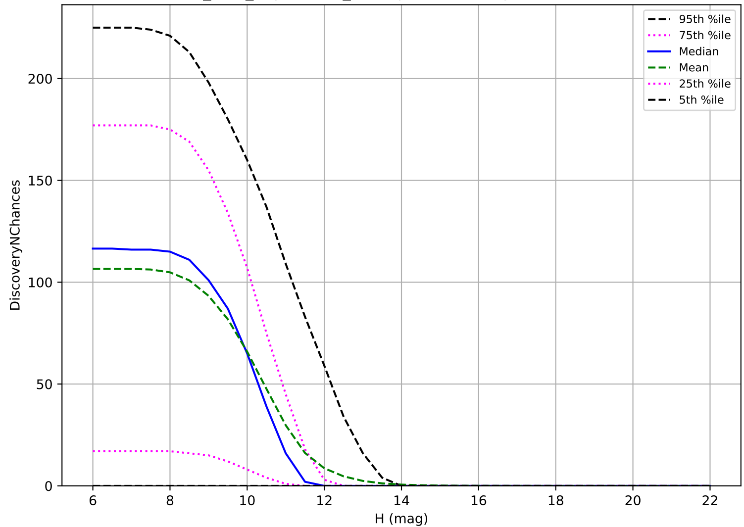
roman_v3.3_10yrs: OCC_r20 3 pairs in 15 nights detection loss
