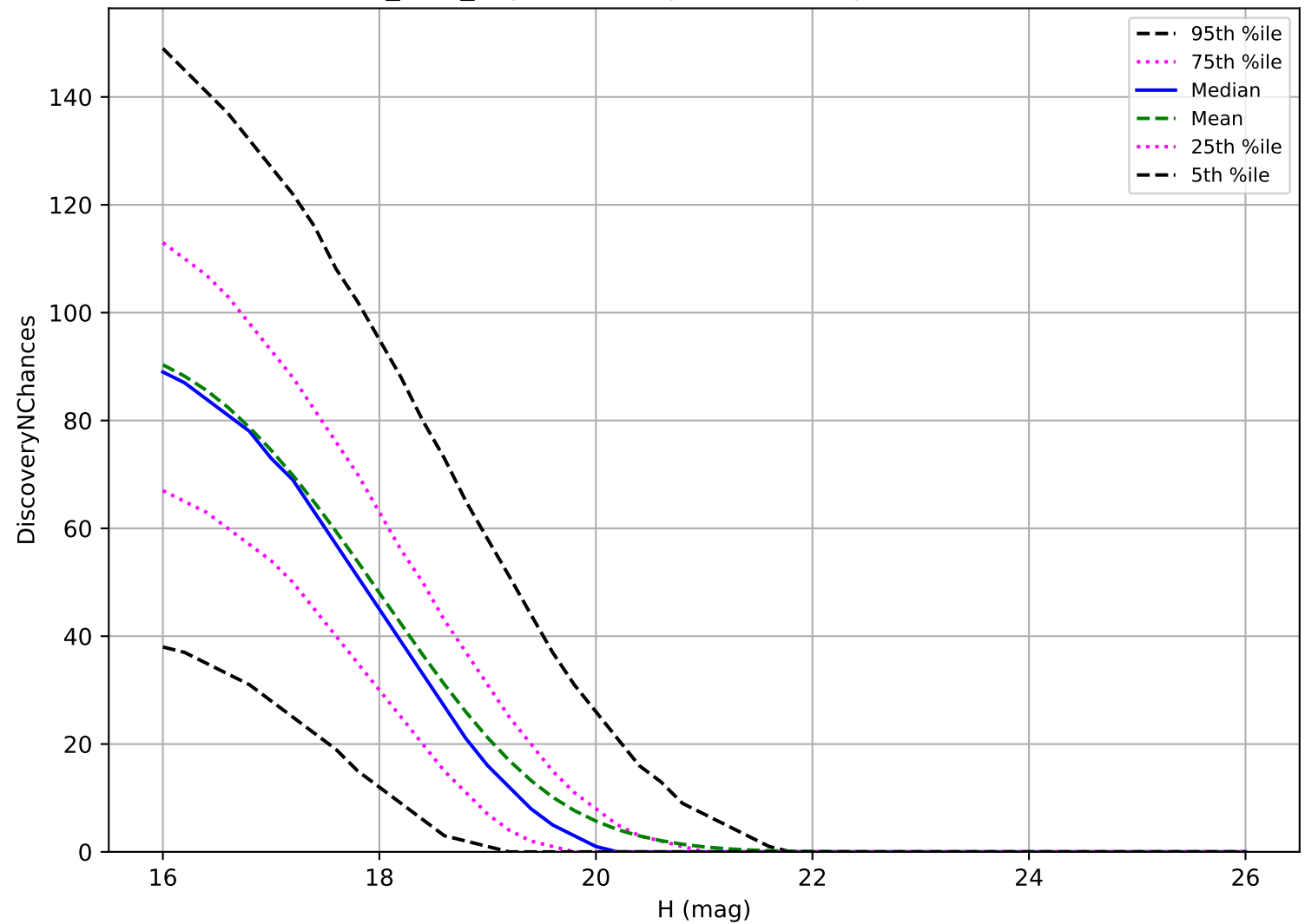
roman_v3.3_10yrs: MBA 3 pairs in 15 nights detection loss
