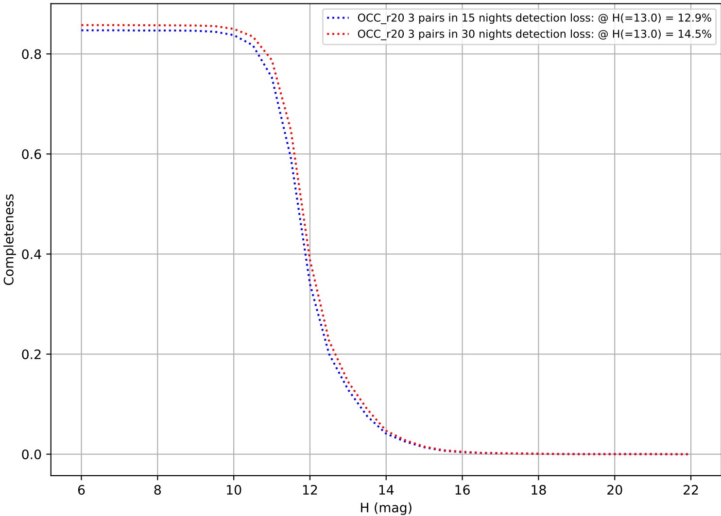
roman_v3.3_10yrs: DifferentialCompleteness
