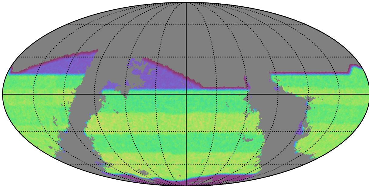
roman_v3.3_10yrs gri band non-DD: riz_exposure_time_year9
