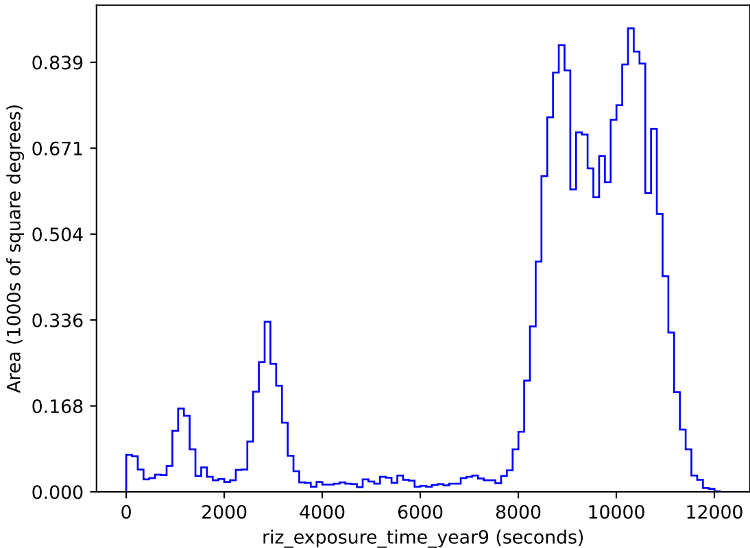
roman_v3.3_10yrs gri band non-DD: riz_exposure_time_year9
