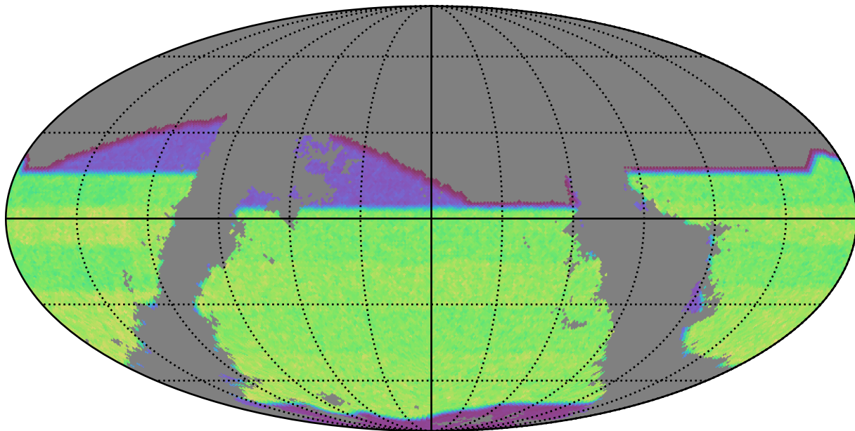
roman_v3.3_10yrs gri band non-DD: riz_exposure_time_year8
