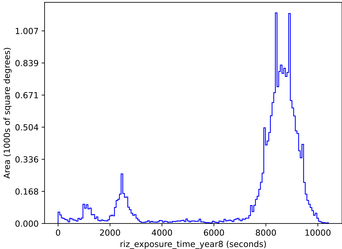
roman_v3.3_10yrs gri band non-DD: riz_exposure_time_year8
