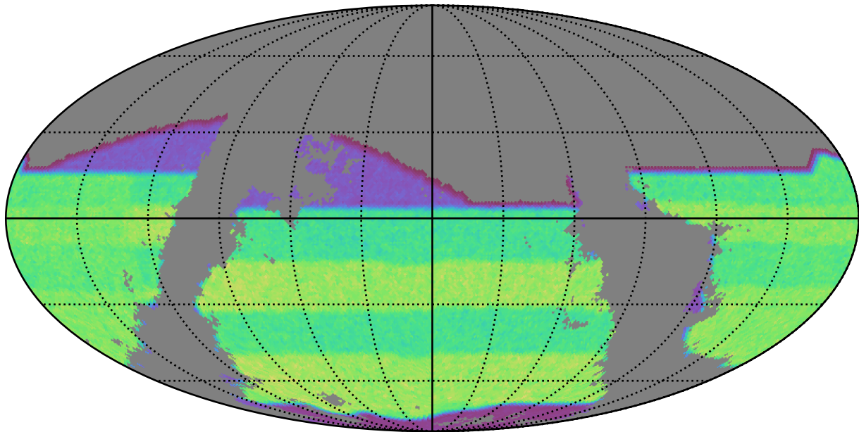
roman_v3.3_10yrs gri band non-DD: riz_exposure_time_year7
