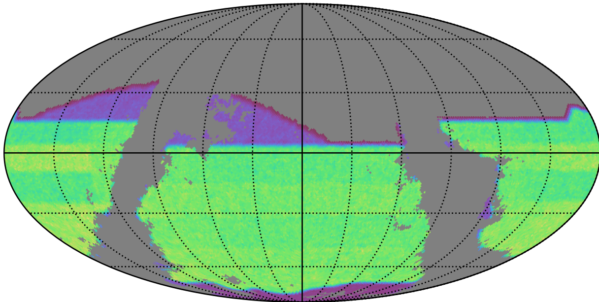
roman_v3.3_10yrs gri band non-DD: riz_exposure_time_year6
