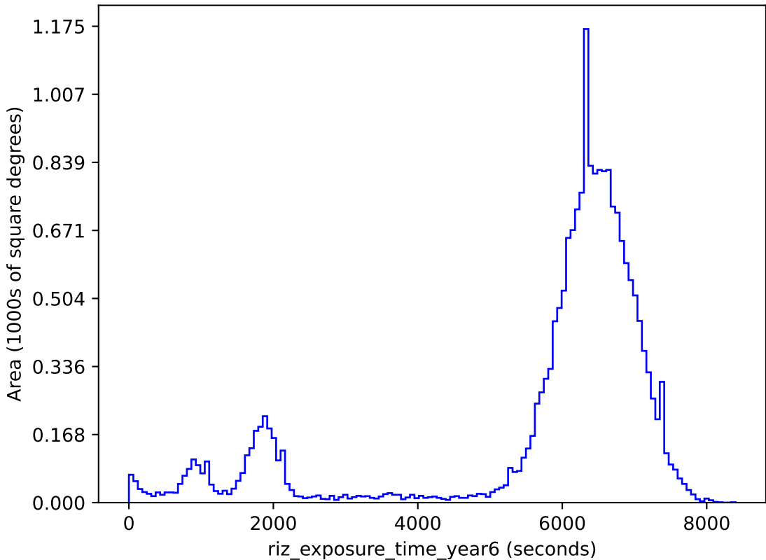
roman_v3.3_10yrs gri band non-DD: riz_exposure_time_year6
