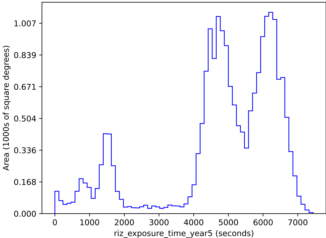
roman_v3.3_10yrs gri band non-DD: riz_exposure_time_year5
