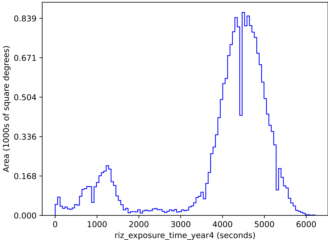
roman_v3.3_10yrs gri band non-DD: riz_exposure_time_year4
