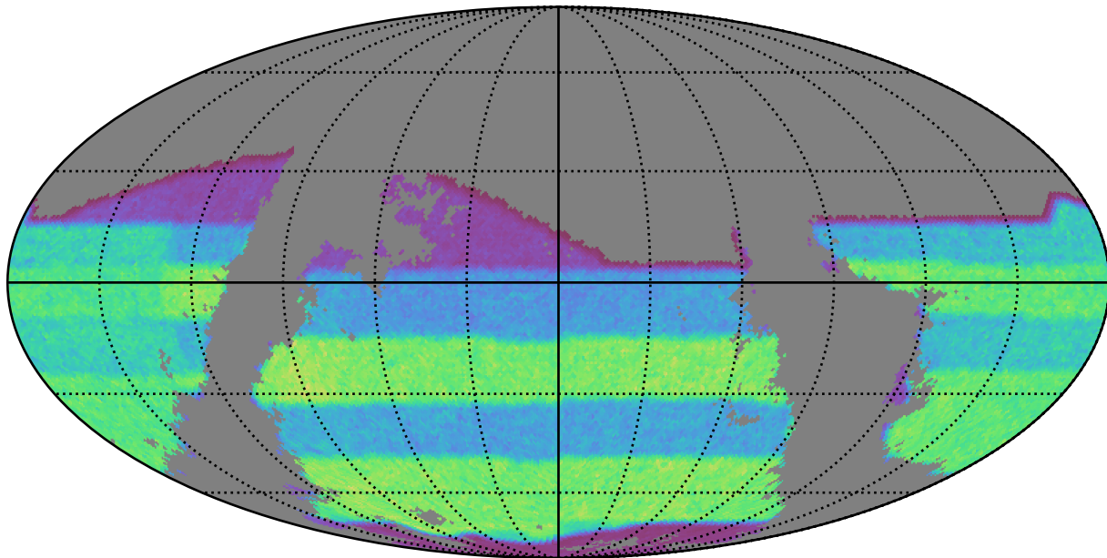
roman_v3.3_10yrs gri band non-DD: riz_exposure_time_year3
