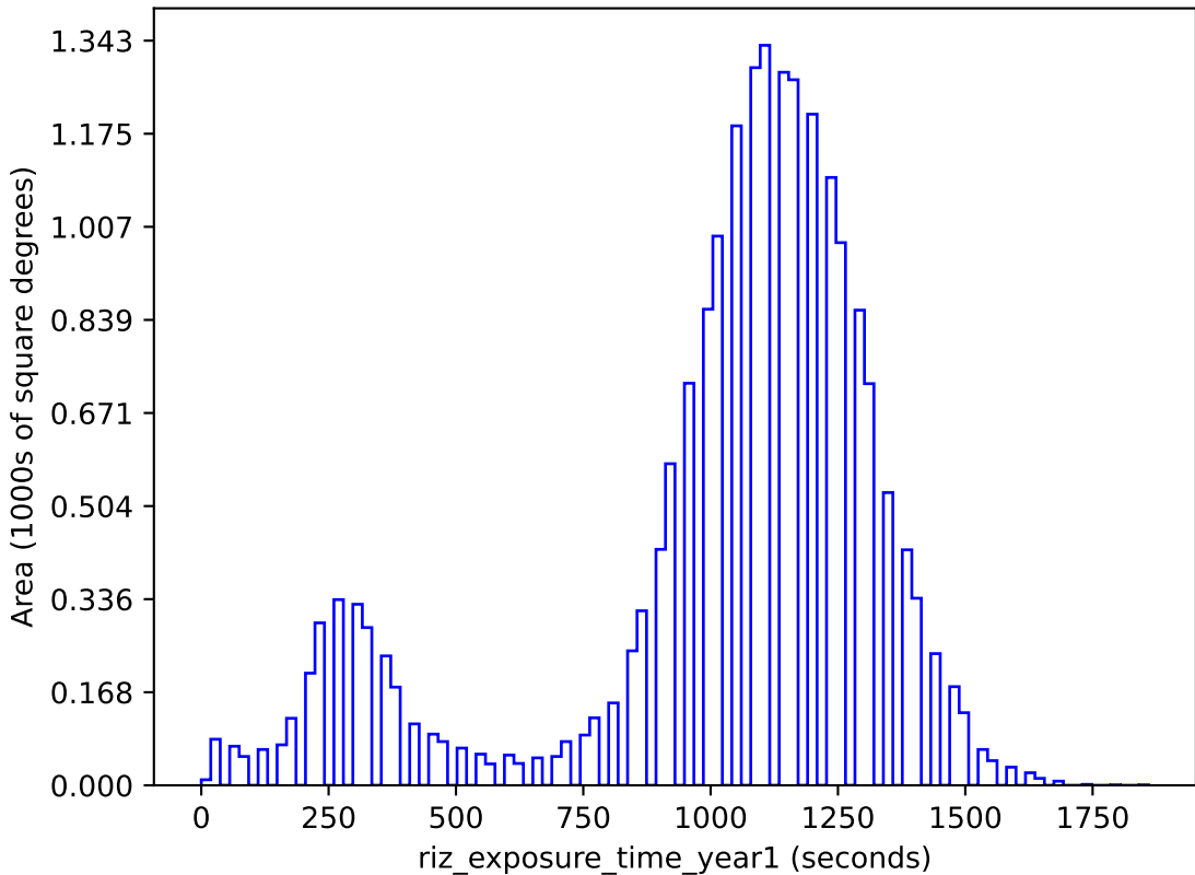
roman_v3.3_10yrs gri band non-DD: riz_exposure_time_year1
