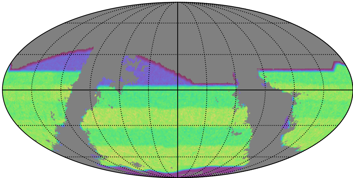
roman_v3.3_10yrs gri band non-DD: gri_exposure_time_year9
