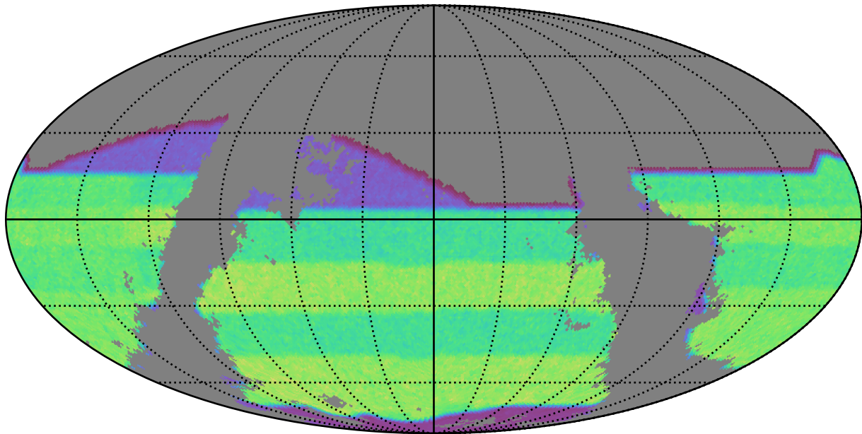
roman_v3.3_10yrs gri band non-DD: gri_exposure_time_year7
