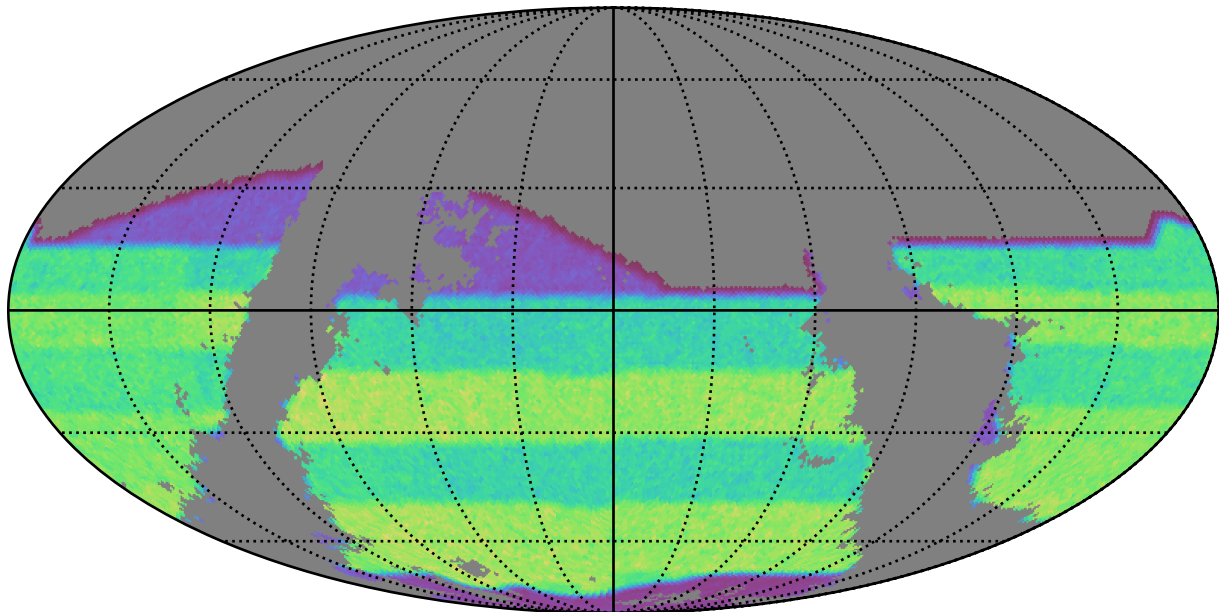
roman_v3.3_10yrs gri band non-DD: gri_exposure_time_year5
