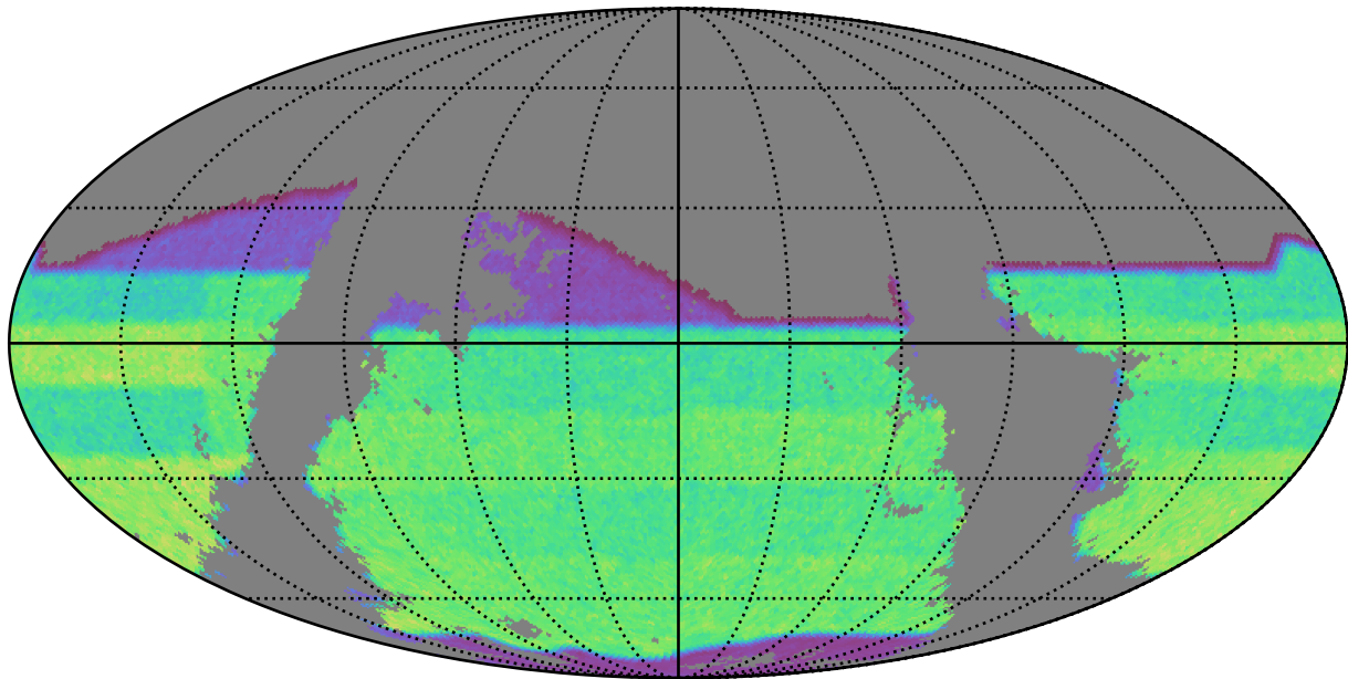
roman_v3.3_10yrs gri band non-DD: gri_exposure_time_year4
