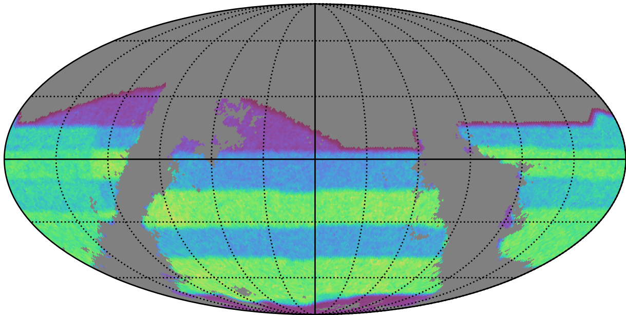
roman_v3.3_10yrs gri band non-DD: gri_exposure_time_year3
