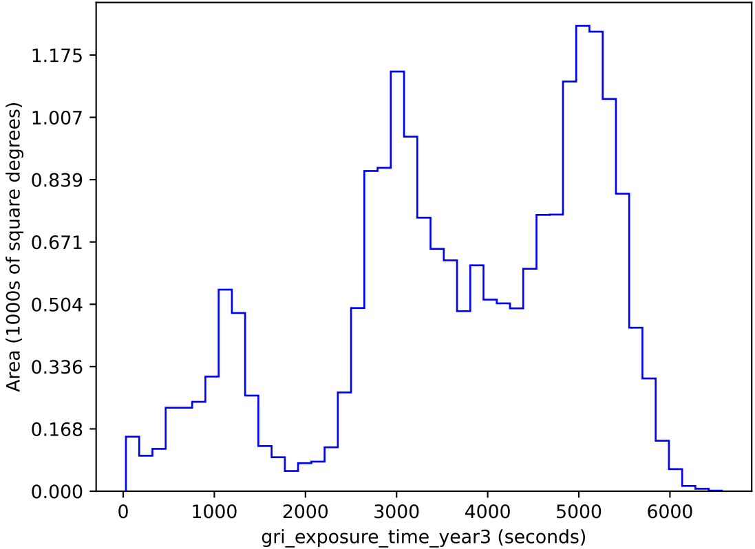
roman_v3.3_10yrs gri band non-DD: gri_exposure_time_year3
