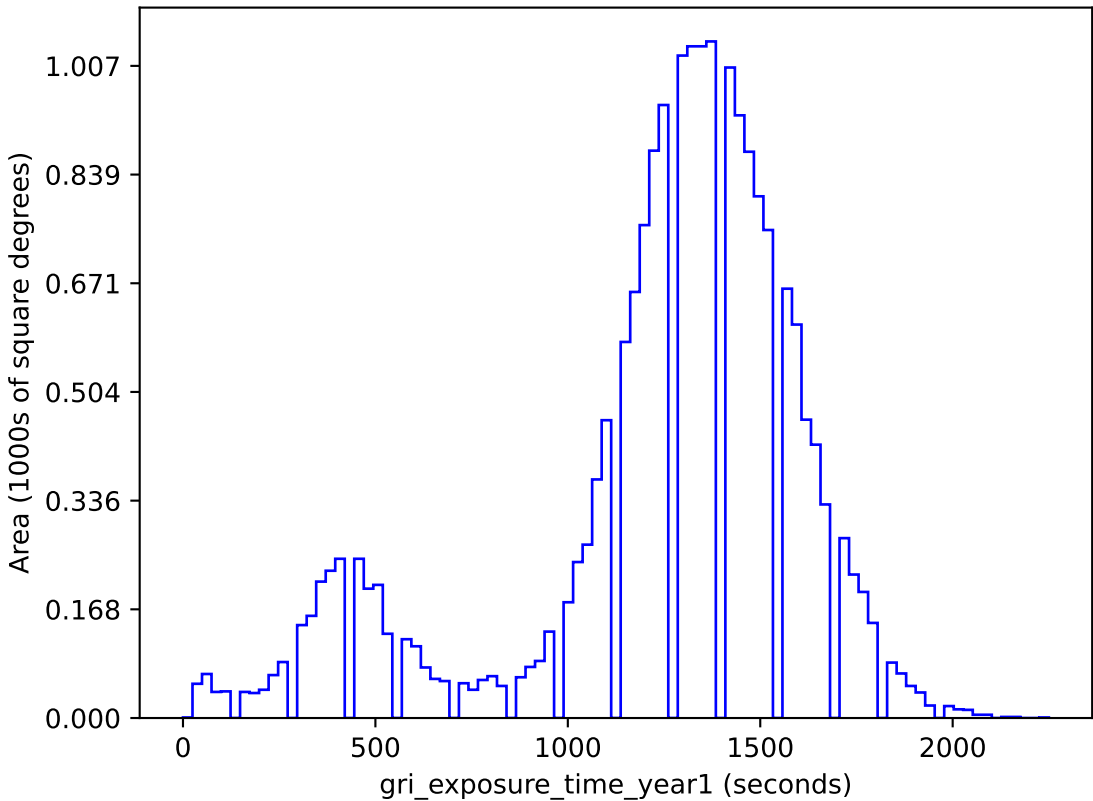
roman_v3.3_10yrs gri band non-DD: gri_exposure_time_year1
