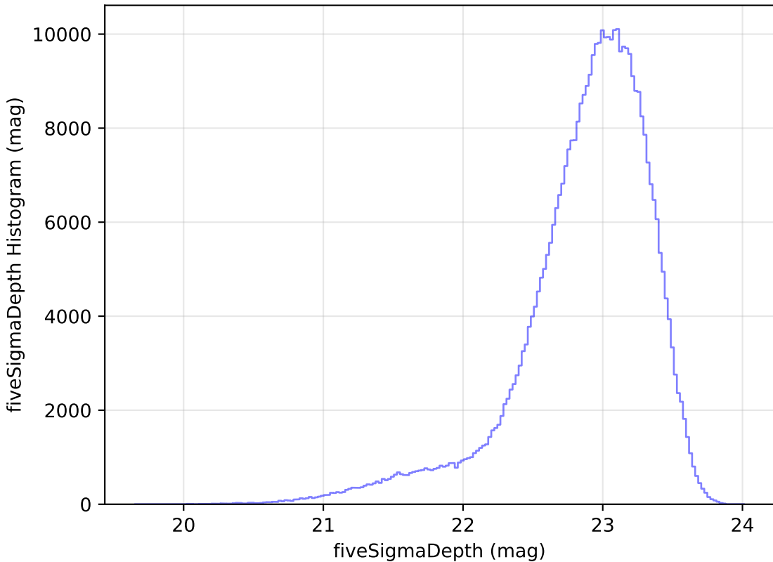
roman_v3.3_10yrs z: fiveSigmaDepth Histogram
