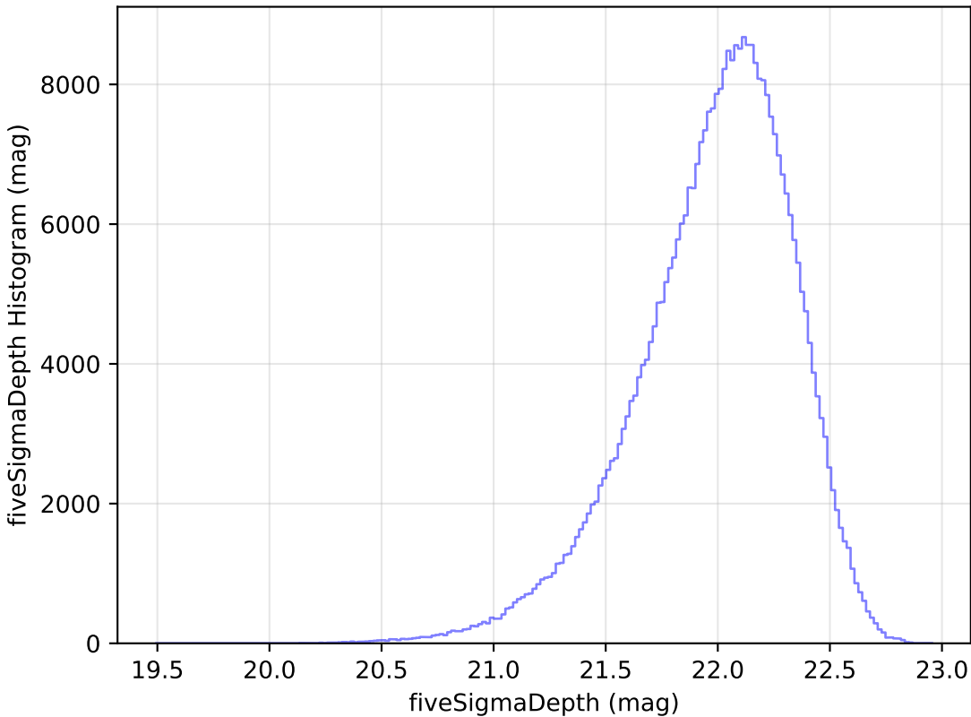
roman_v3.3_10yrs y: fiveSigmaDepth Histogram
